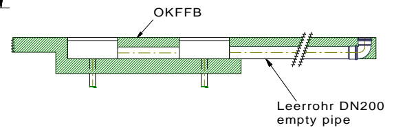
Detail "Y"
