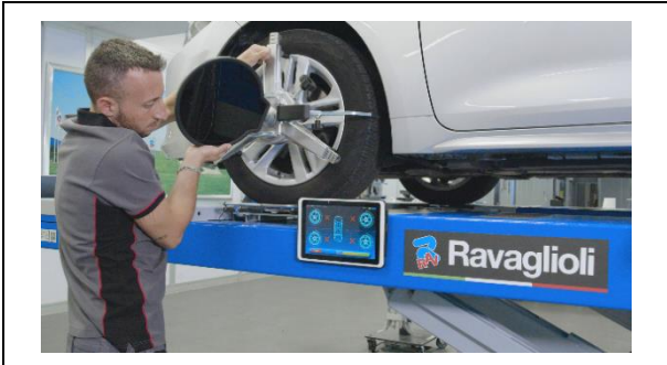
Wheel-aligner-RAV3D2.0WALL-tablet-DI
